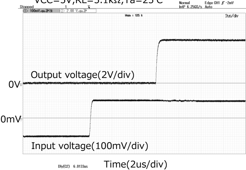
Rise response time VCC=5V,RL=5.1k \Omega ,Ta=25 ^{\circ} C
