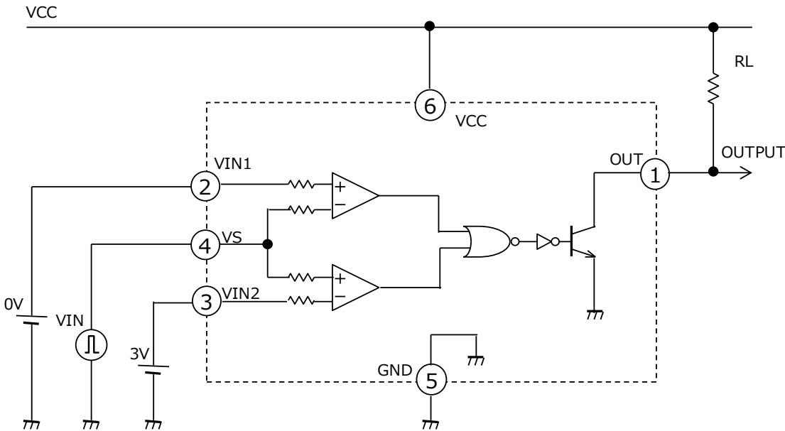
Response time measurement circuit
