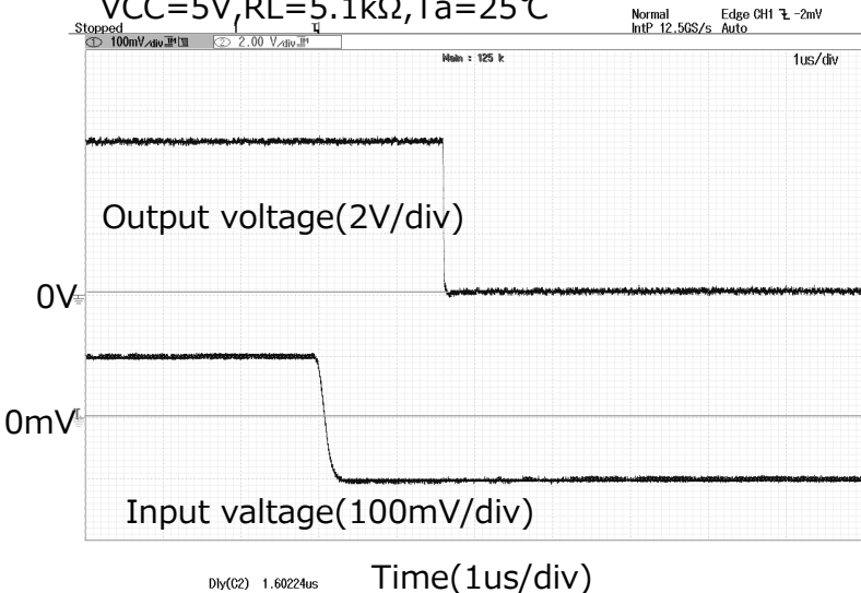
Fall response time VCC=5V,RL=5.1k \Omega ,Ta=25 ^{\circ} C
